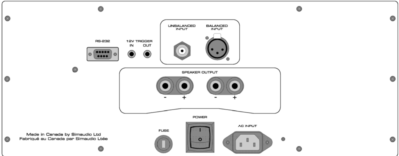
Figure 1: Rear panel of Moon 880M Mono Amplifier
